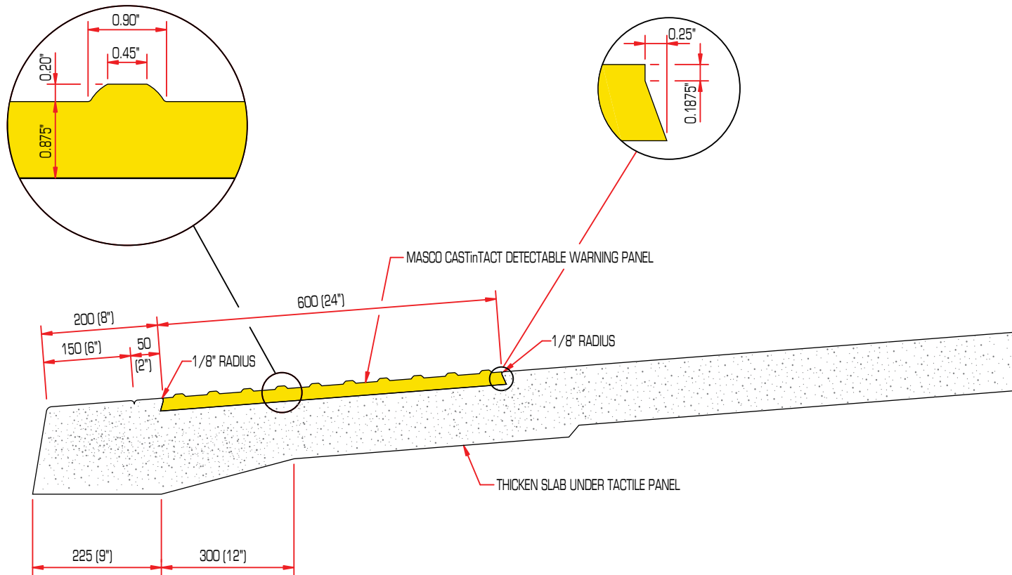
CROSS SECTION OF DETECTABLE WARNING PANEL
