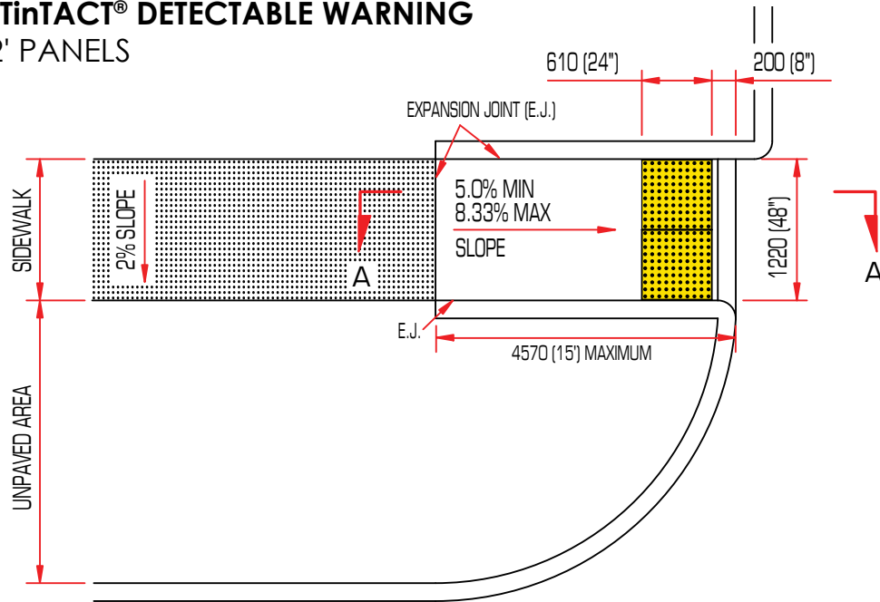
1220mm (48") PARALLEL SIDEWALK RAMP DETAIL OPTION 2
