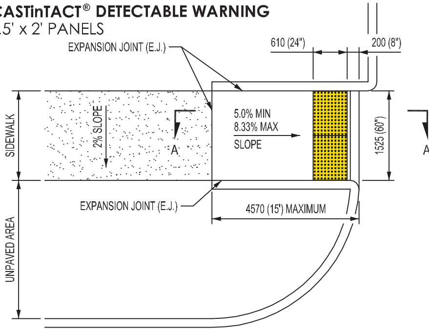
1525mm (60") PARALLEL SIDEWALK RAMP DETAIL OPTION 2
