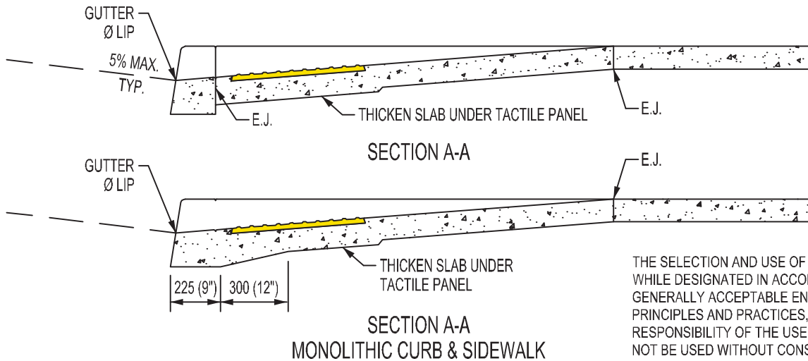
1525mm (60") PARALLEL SIDEWALK RAMP DETAIL OPTION 2
