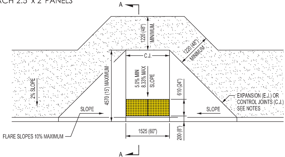
1525mm (60") PERPENDICULAR SIDEWALK RAMP DETAIL OPTION 3
