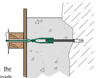
SC with Drop-in anchor
