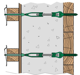
SC's used with Coil-Lags™ attached to wood lagging
